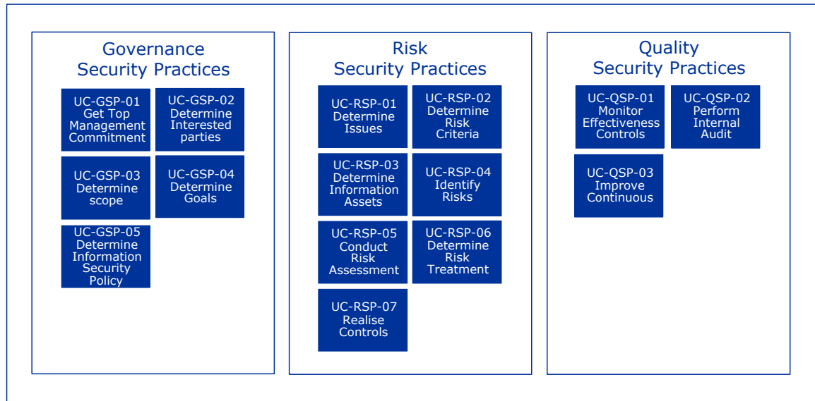
Figure 1, Information security practices.
