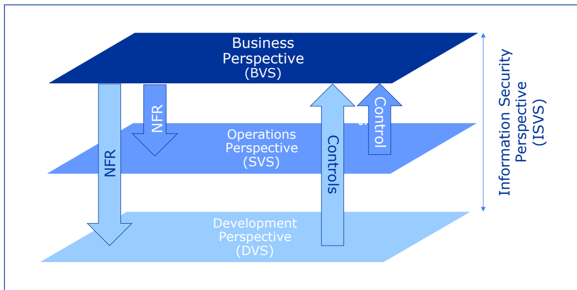
Figure 4, ISVS as integrator of the BVS, SVS and DVS.
